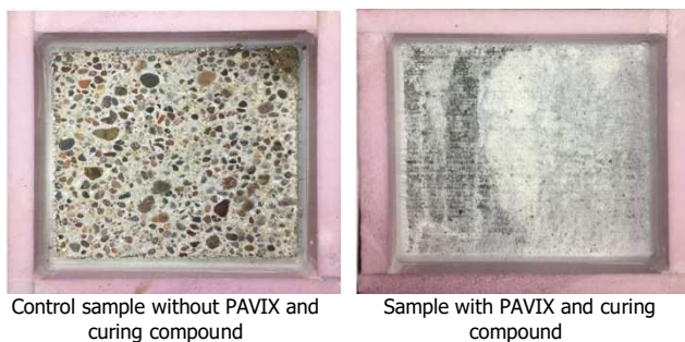
Fig. 4-a: ASTM C672-98: scaling resistance when PAVIX is applied on green concrete surfaces exposed to deicing chemicals, this test shows 94% reduction in mass loss at 70 Freeze-Thaw cycles.
